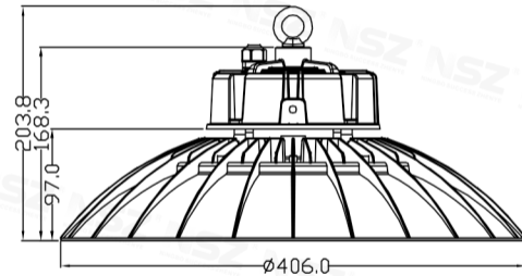
ZY-8008N-DC 200/240W
