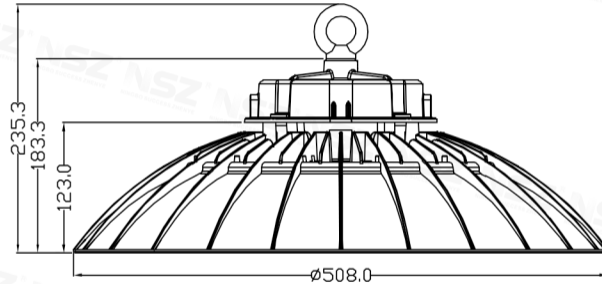
ZY-8008N-DC 400/500W
