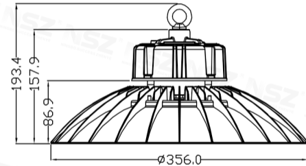
ZY-8008N-DC 100/150W
