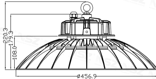
ZY-8008N-DC 300W
